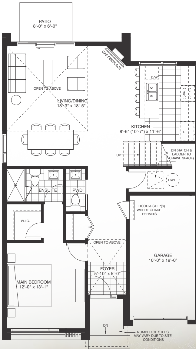
MAIN FLOOR
