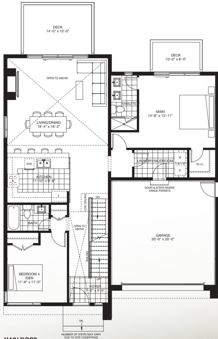
MAIN FLOOR
