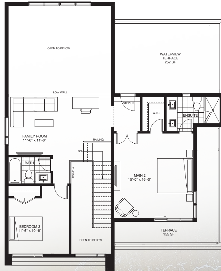
SECOND FLOOR
