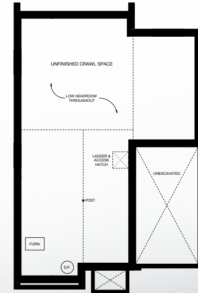
CRAWL SPACE (UNFINISHED) *WHERE BASEMENT IS NOT PERMITTED
