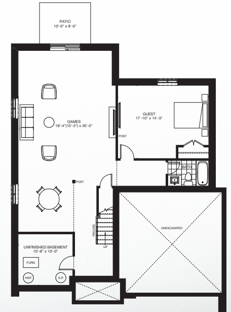
OPT. FINISHED BASEMENT (1,183 SF)
