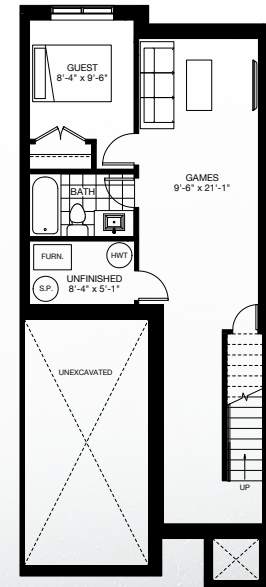
OPT. FINISHED BASEMENT (542 SF)
