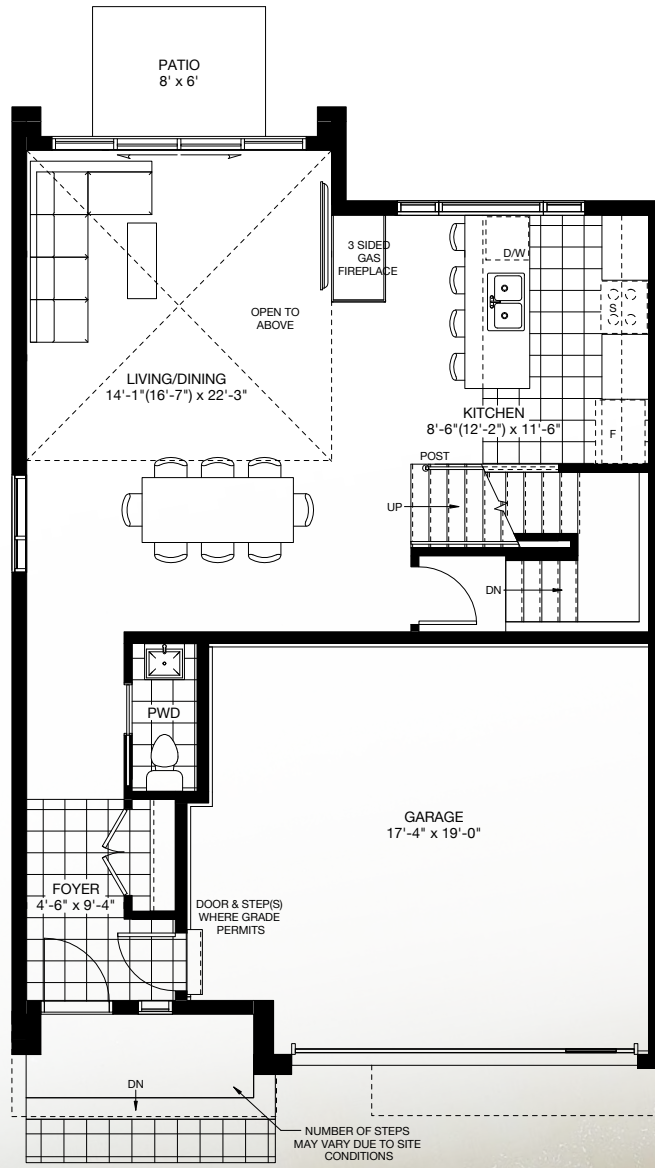
MAIN FLOOR
