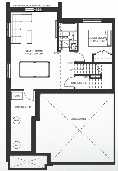
OPT. FINISHED BASEMENT (552 SF)
