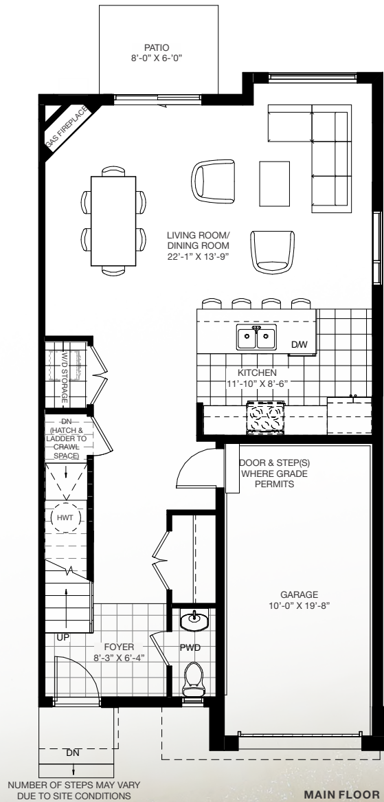
MAIN FLOOR
