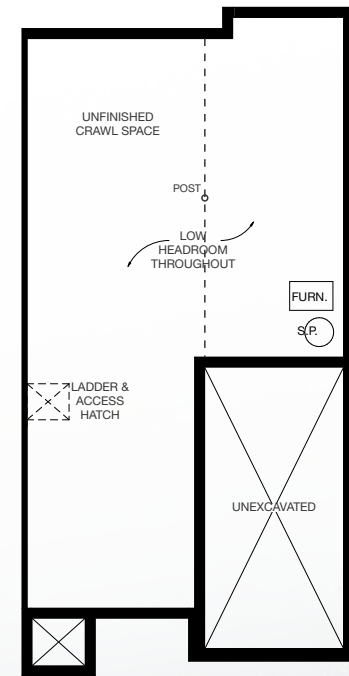
CRAWL SPACE (UNFINISHED) *WHERE BASEMENT IS NOT PERMITTED
